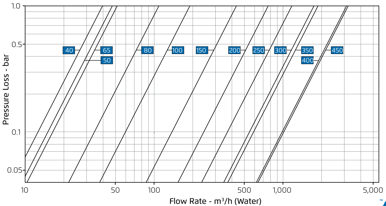
700 Angle Pattern, Throttling Plug (V-Port)
