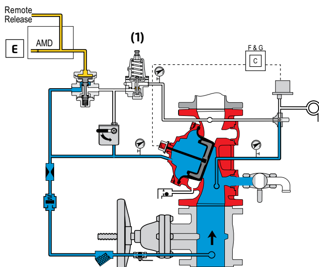
Fig 3a - Valve Closed (Normal Conditions)
