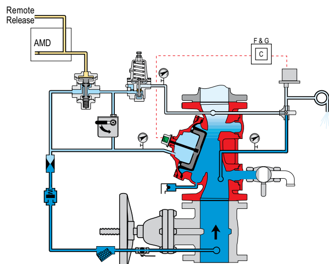
Fig 3b - Valve Open (Fire Conditions)
