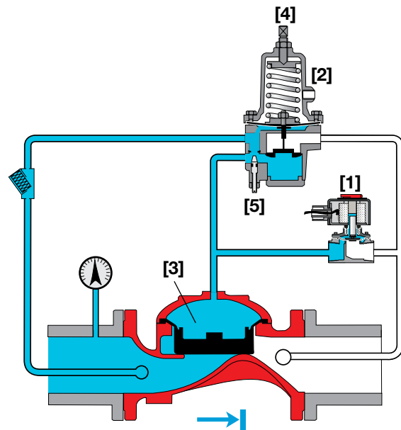
6" - 12" Configuration (Close)
