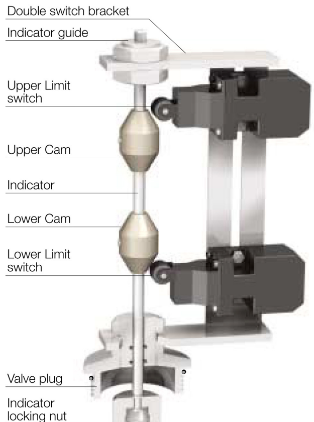
Double limit switch assembly
