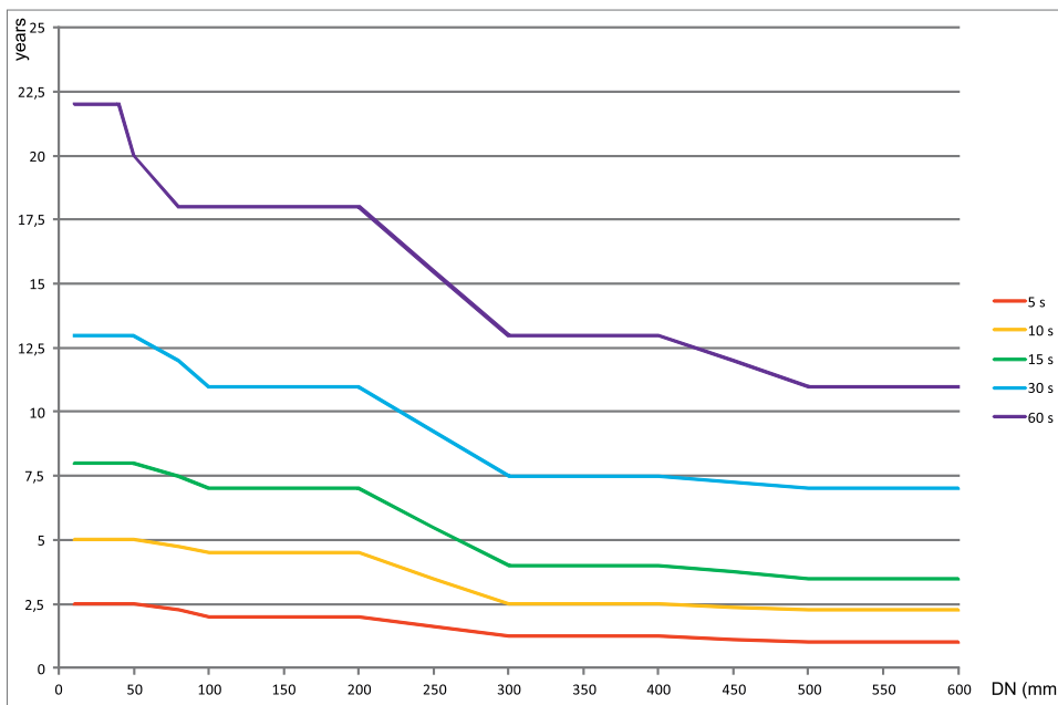
Expected battery life (years) VS sensor diameter and sampling time
