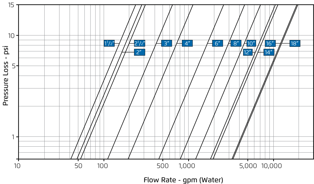
700 Angle Pattern, Flat Disc
