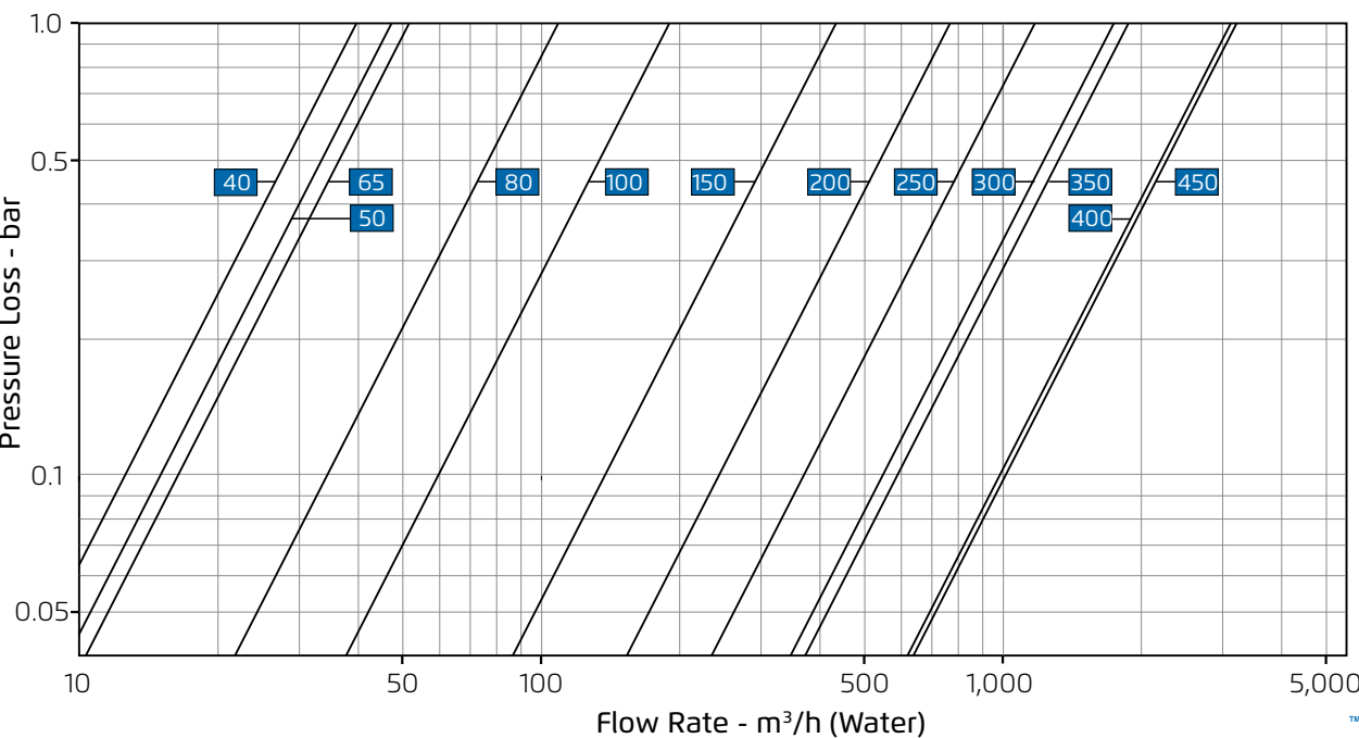
700 Angle Pattern, Throttling Plug (V-Port)
