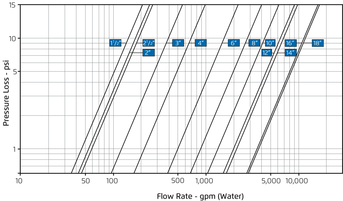
700 Angle Pattern, Throttling Plug (V-Port)
