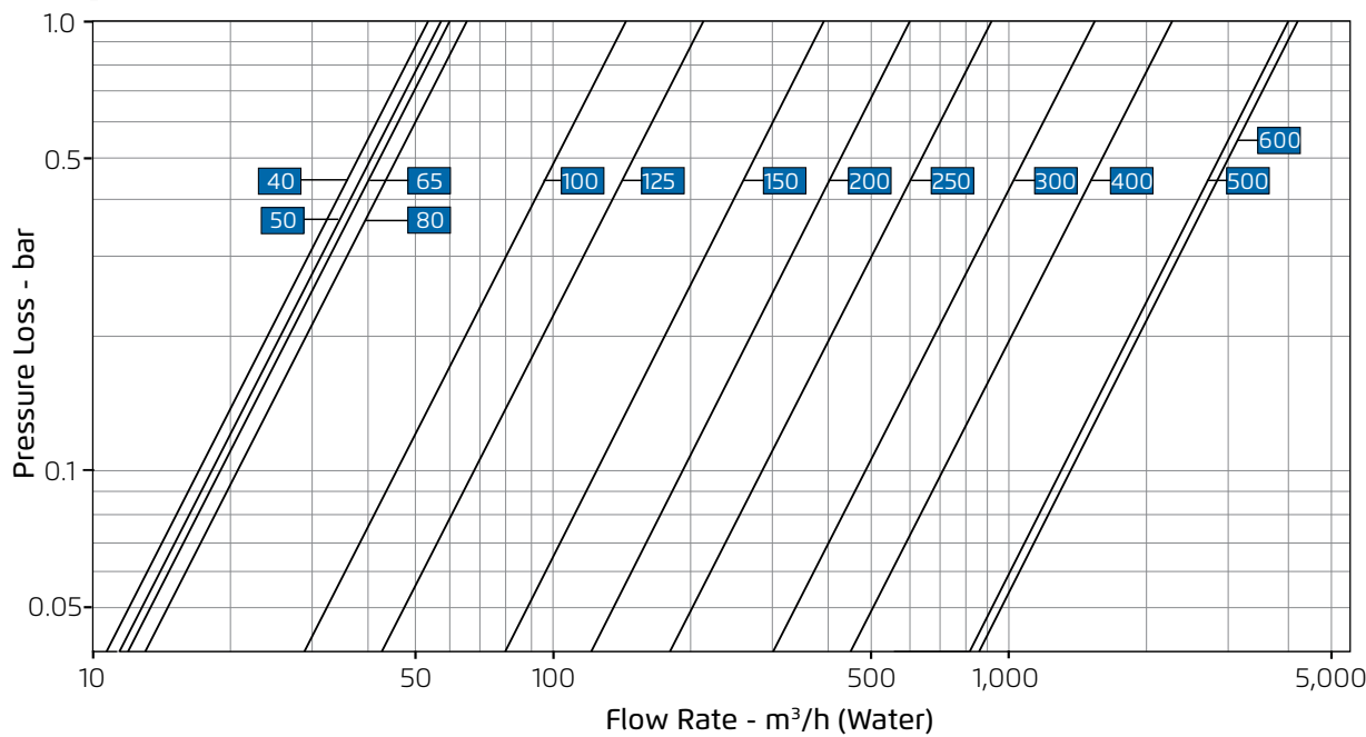
700-ES "Y" Pattern, Flat Disc
