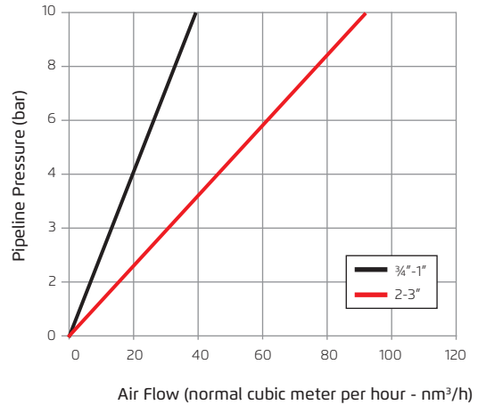
Air Release (Pressurized Operation)
