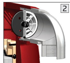
Surge Protection (anti slam) - (2"/3"-C10-SP)
