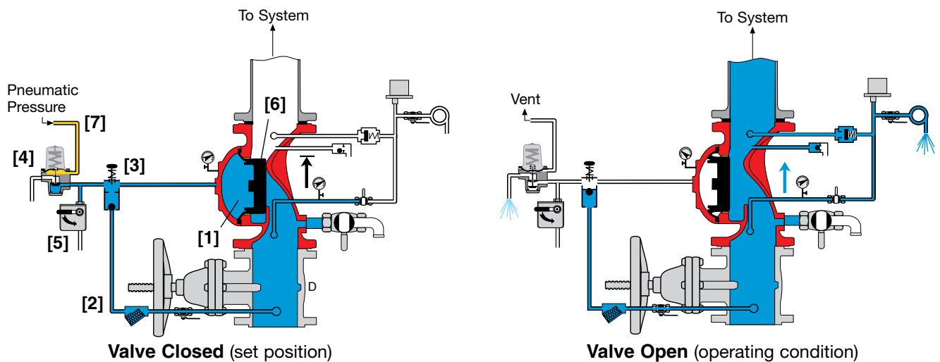
Figure 2: Operation Drawing
